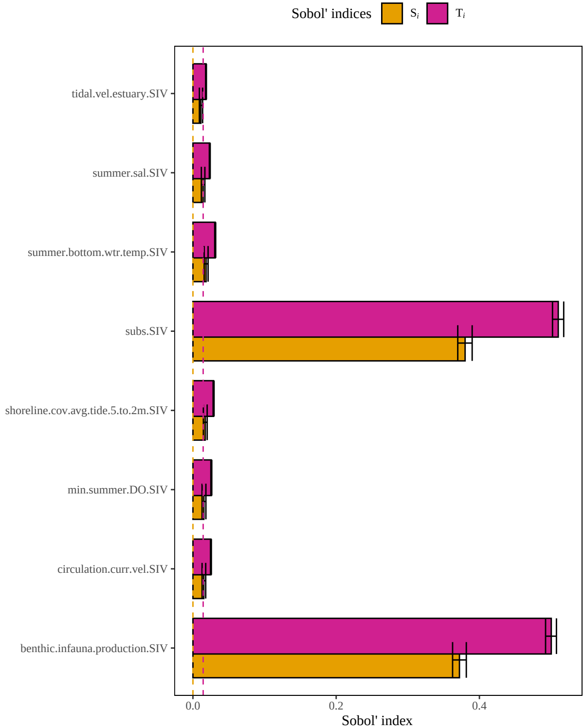
Figure 5. Results of a sensitivity analysis for the southernkingfishEstu model based on a geometric mean structure. Dashed lines represent baseline numerical approximation error for S_i and T_i ( i.e. , dummy variables).
